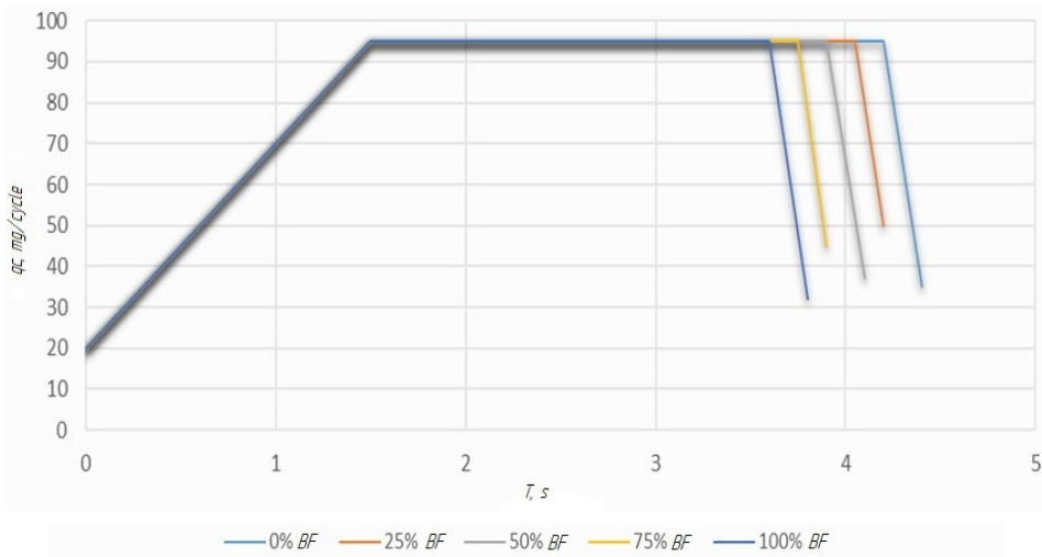
Fig. 5. Dependence of the cyclic supply of the fuel mixture q_t with different percentage composition on time T during acceleration of the diesel engine crankshaft
