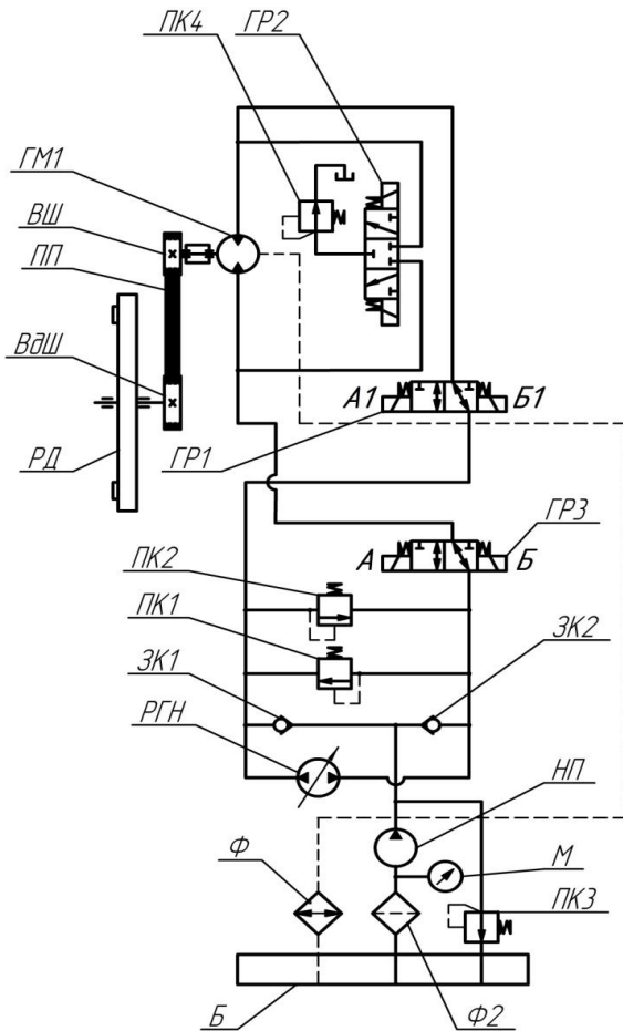
Fig. 4. Structural and functional scheme of the mechanism.
