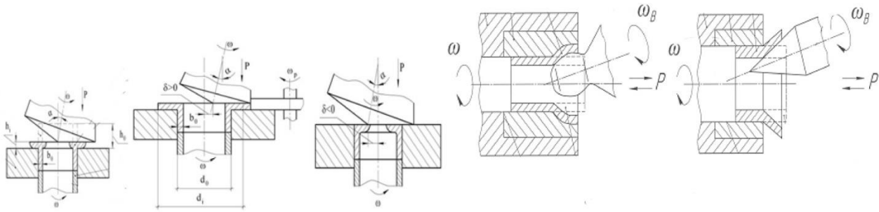
Fig. 2. Influence of the direction of displacement of the peak of the roll of the axis of the workpiece on the shape change of the workpiece during the loading of the clamps by the method of RS
