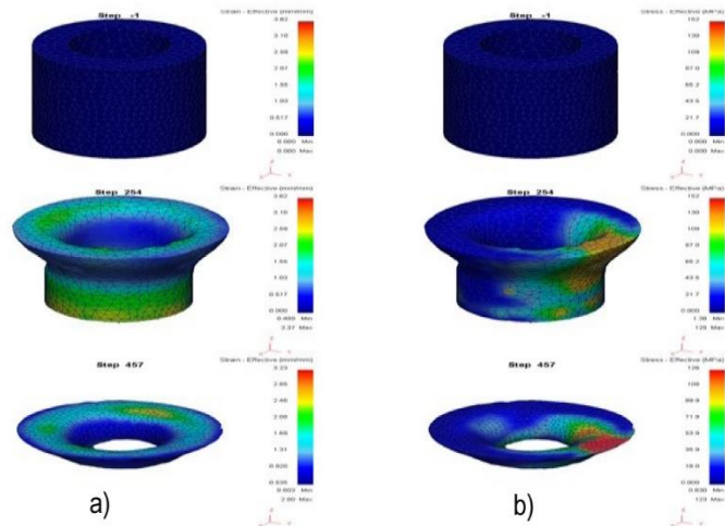
Fig.15 Distribution of accumulated deformation:a) intensity of stresses; b) during modeling of the RS process of lead sample.
