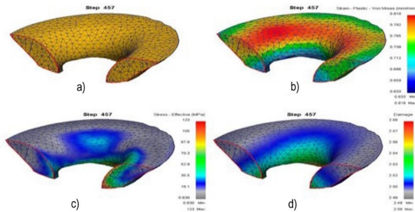
Fig.18 Analysis of VAT modeling results: form change a); distribution in the midinary section of the pipe workpiece at the final stage of the RS accumulated deformation b); intensity of stress in); accumulation of damage d).
