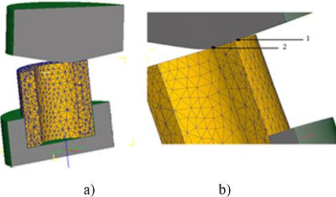
Fig. 10. The finite element method of RS flanging modeling for the outer clamp on the tube workpiece: a) calculation model; b) the location of the calculation points 1 and 2 [11].
