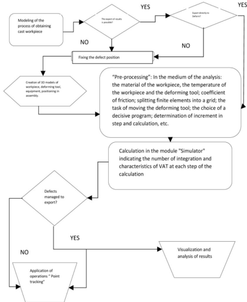
Fig. 4. Algorithm for the simulation of through technological processes in software complexes of finite-element modeling of the DEFORM-3D type
