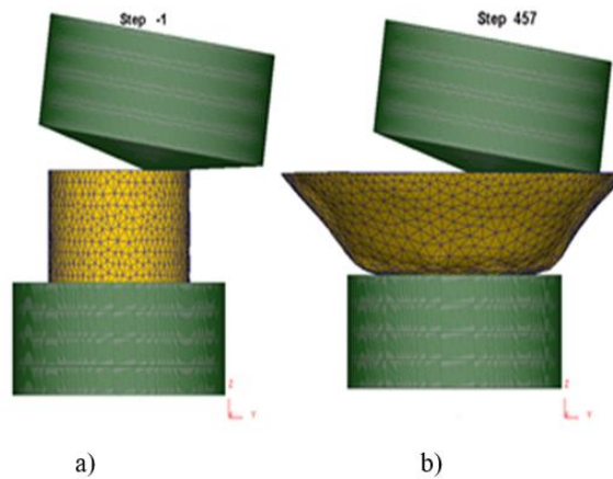
Fig. 5. Scheme of the RS process: a - initial position; b - at the moment of the established stage.
