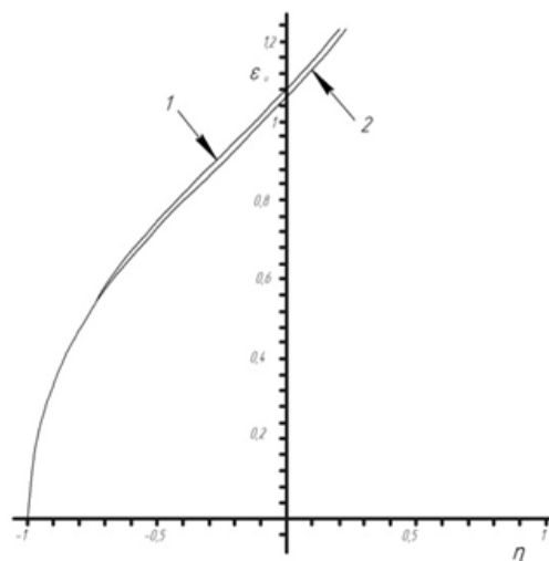
Fig.17 Trajectory of deformation of the lateral surface of lead sample number 5: 1-experimental study; 2- modeling in the software package DEFORM-3D[8]
