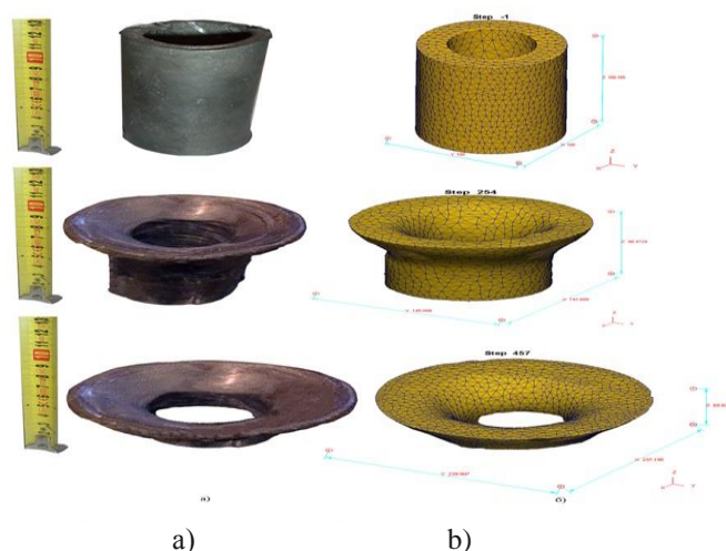
Fig.14 RS of a lead workpiece №5: a) experimental research; b) modeling in DEFORM 3D[7].
