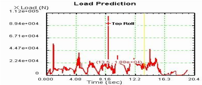
Fig. 8. Dependence of the RS's efforts on the Poisson movement (roller)
