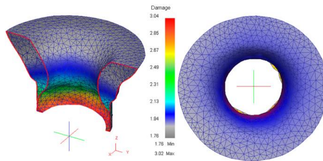
Fig. 6. The distribution of damage \Psi_i in the volume of deformed metal
