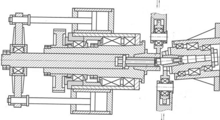
Fig. 1. Prefabrication for implementation of rolling stamping processes.
