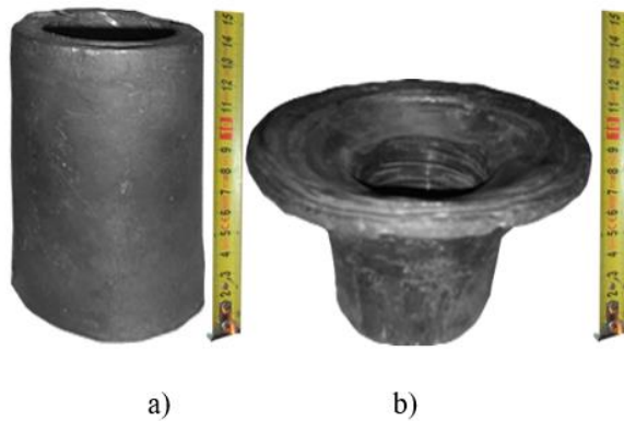
Fig. 11. Lead workpiece № 1 before RS (a) and after RS research (b).
