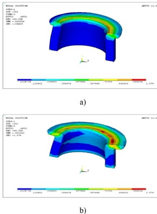
Fig. 12. The nature of the formation of the external clamp and the distribution of the zones of intensity of deformation in it for different degrees of upsetting by rolling a) and b) with arbitrary placement of the workpiece in the matrix.
