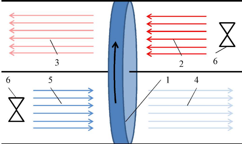
Figure 7. Technological scheme of the regenerative recycler: 1 – heat exchange regenerative surface; directions of air movement; 2 – from the room; 3 – in the external environment; 4 – indoors; 5 – from the external environment; 6 – fan
