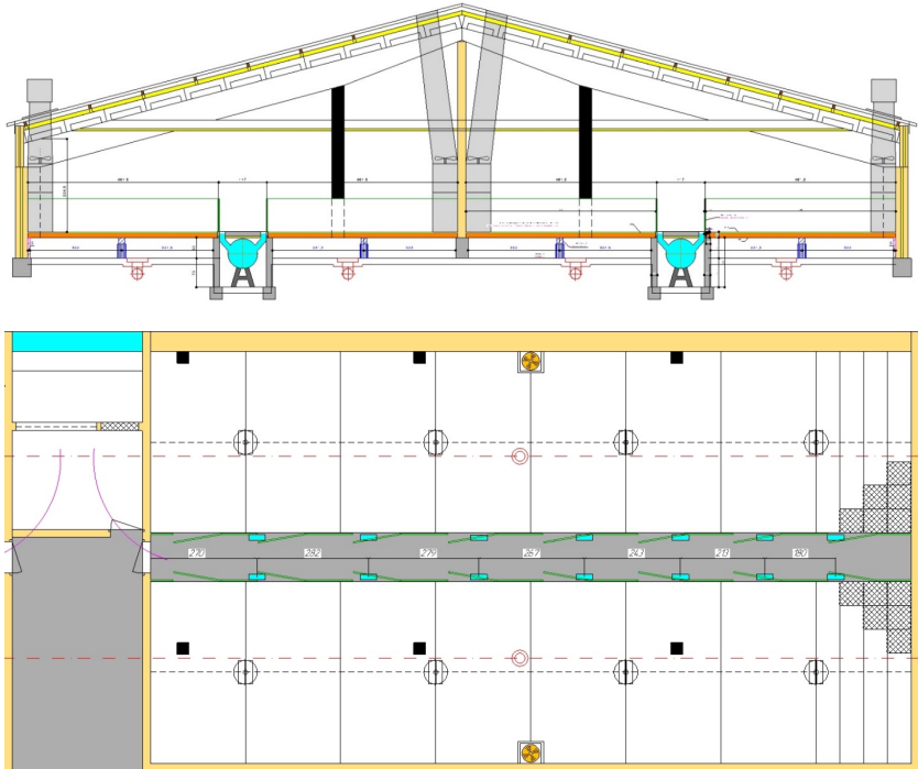
Figure 18. The project of the section of the room for keeping piglets for fattening with a new location of ventilation holes
