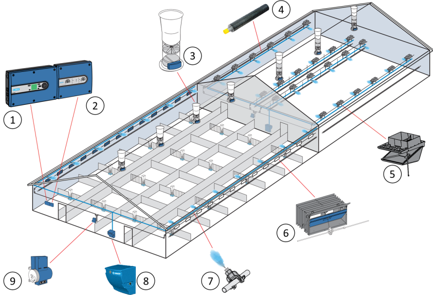
Figure 4. Negative pressure ventilation system:
