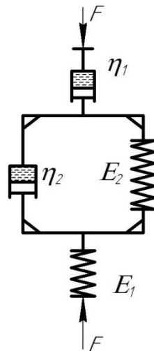
Fig. 2. Rheological model of plant material
