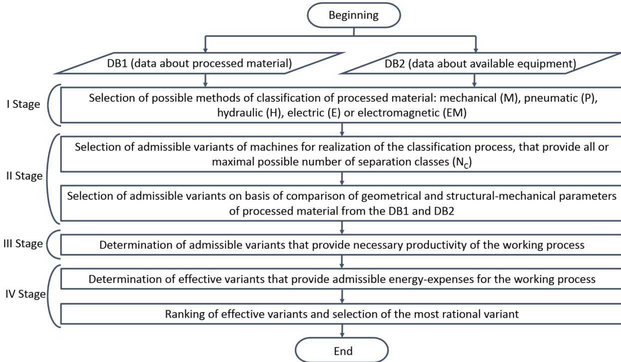
Fig. 1. The block-scheme of an algorithm of the proposed method of automated technological projection of classification processes of dry dispersive materials
